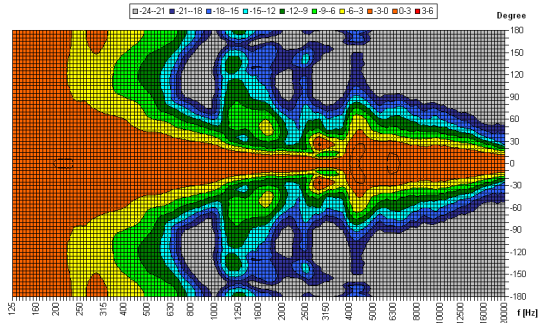
Horizontal Isobars of: Elko-Schmid MHE-50T
