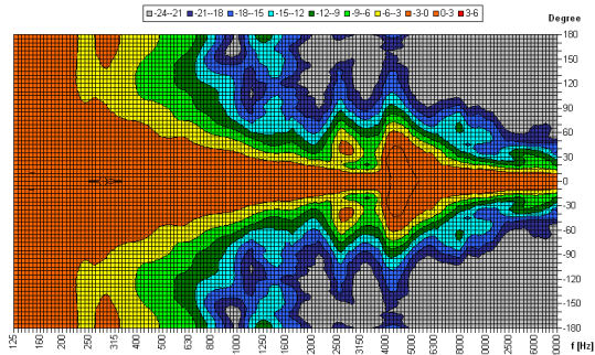
Vertical Isobars of: Elko-Schmid MHE-50T
